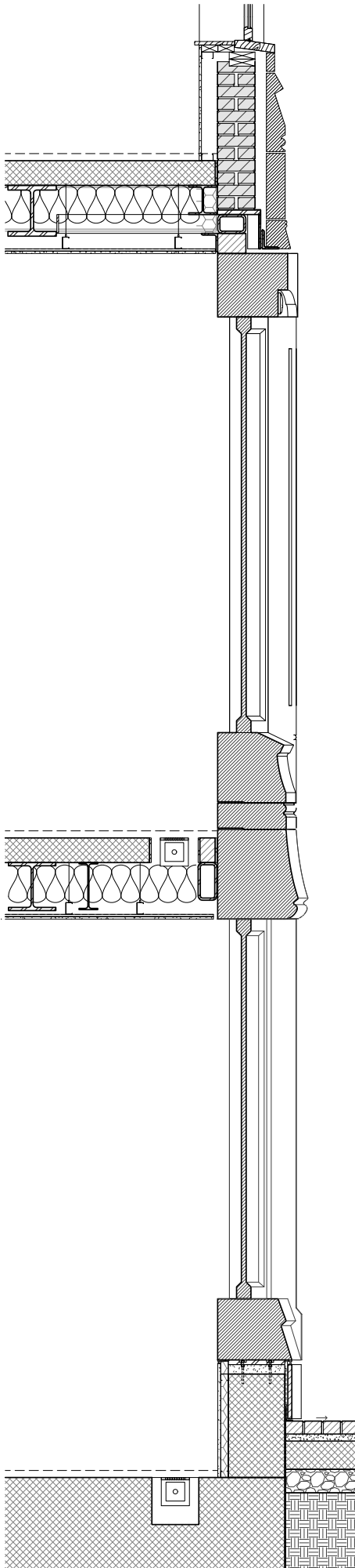
Wall section at storefront windows and entry
